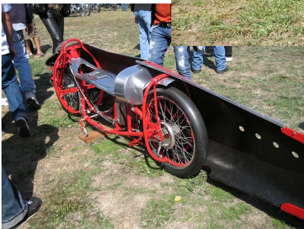
Cut-A-Way
